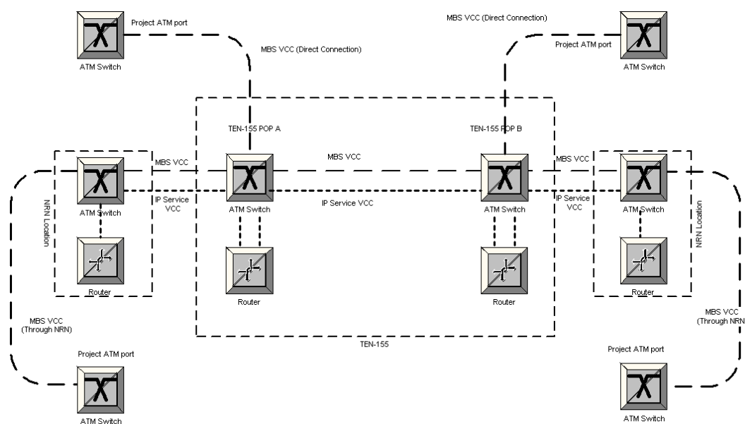
[fig 2] TEN-155 MBS Architecture
