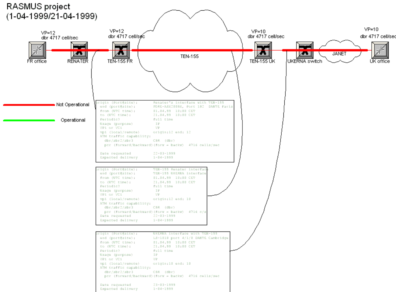
[fig 11] Complete network topology
